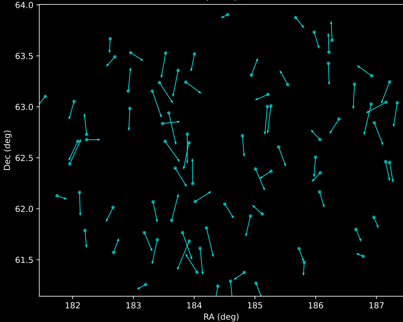
APOGEE DR17 Noise Stream Proper Motion Vectors (n=81)
