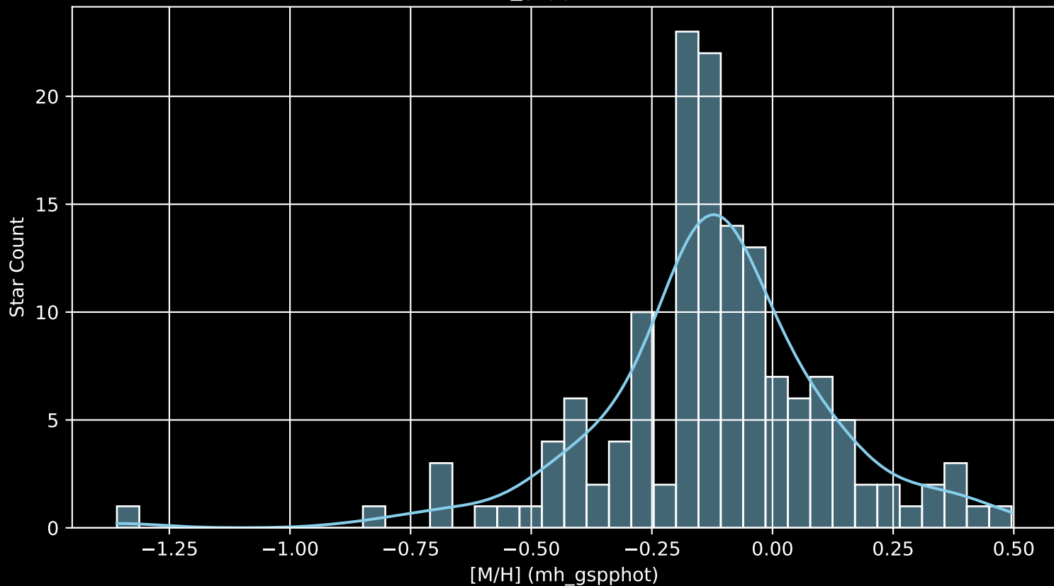
APOGEE DR17 Field: [150+16 [M/H] (mh_gspphot) (n= 145)
