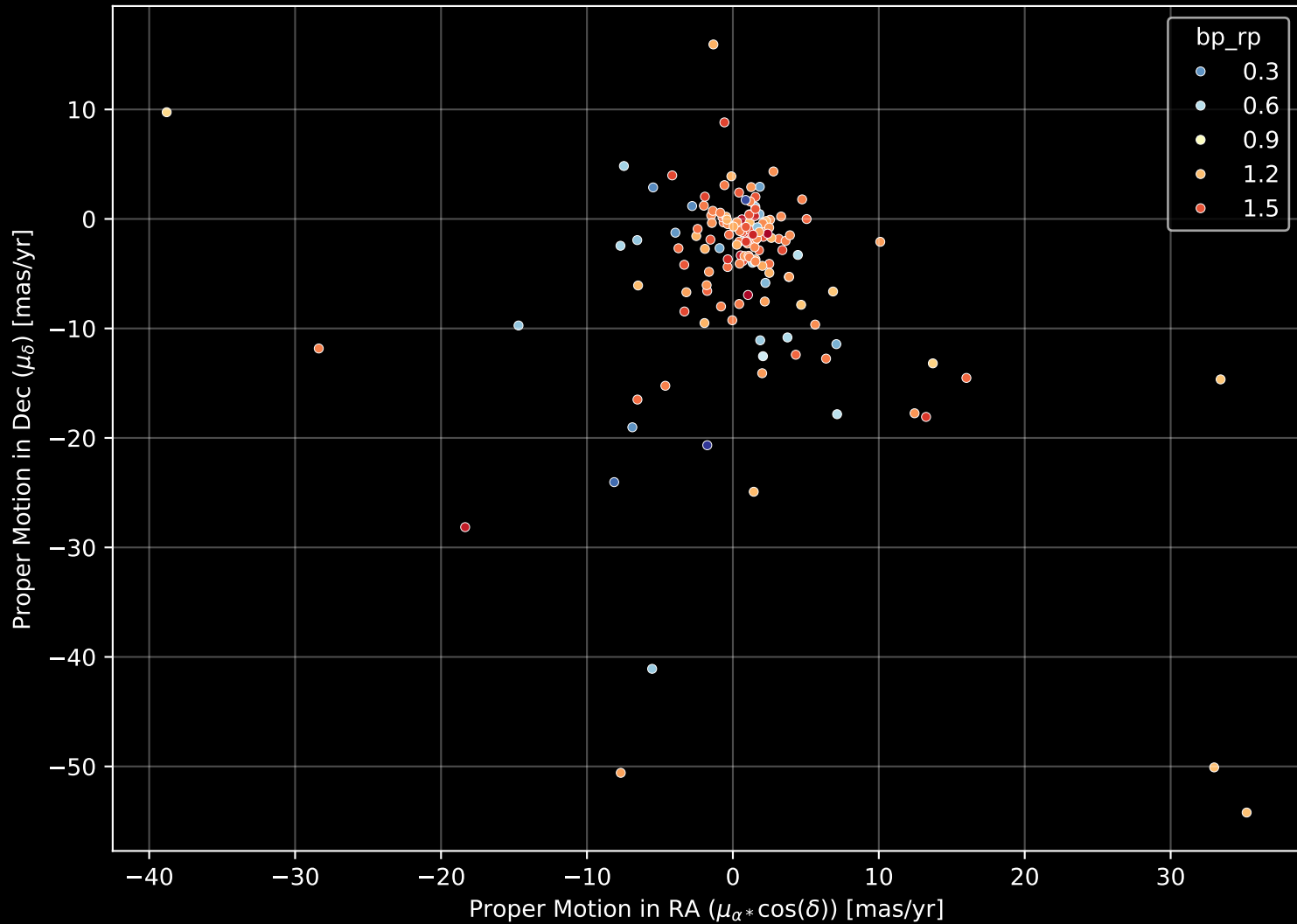
APOGEE DR17 Field: [150+16] Proper Motion Diagram (n= 147)
