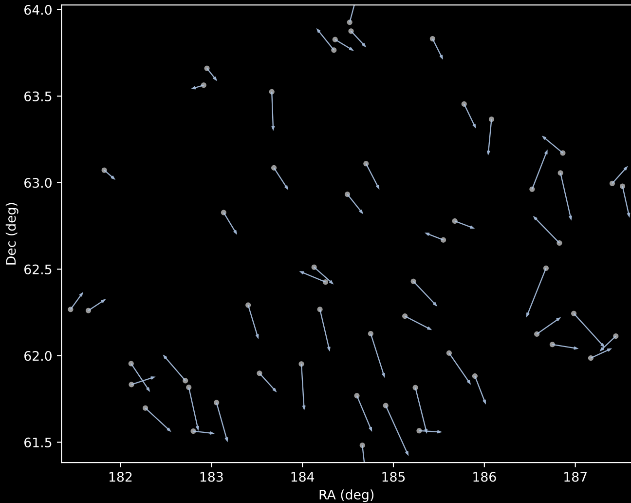
APOGEE DR17 Cluster 1 Proper Motion Vectors (n=54)
