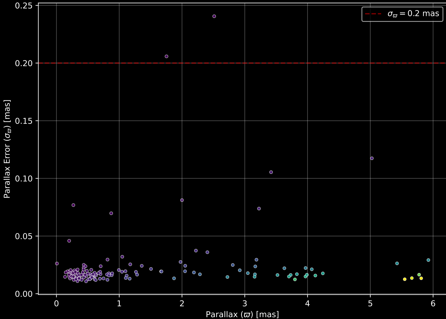
APOGEE DR17 Field: [150+16] Parallax Quality (n= 147)
