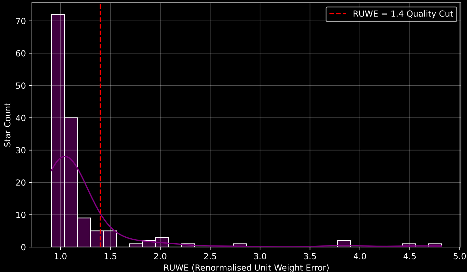
GAPOGEE DR17 Field [150+16] RUWE Distribution (n= 143)
