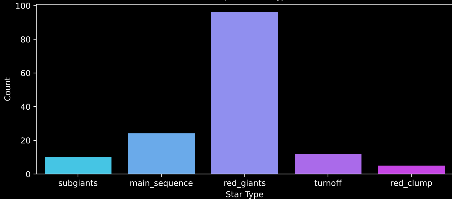
APOGEE DR17 Field: [150+16] Count plot of Star Type
